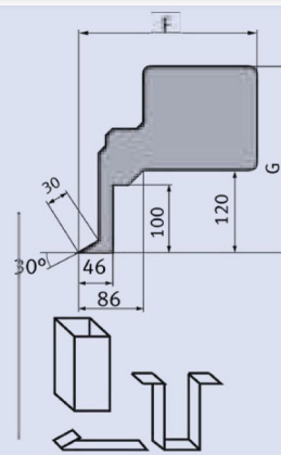
Dimensions Bending beam HSBM SH
